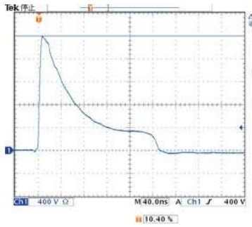
PULSE OUT connector waveform: 50Ω
