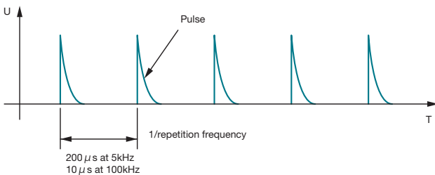
Pulse wave shape into a 50 Ω load and general graph of a fast transient/burst
