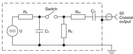
Circuit diagram of a fast transient/burst generator
